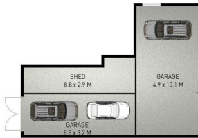
SHED/GARAGE
