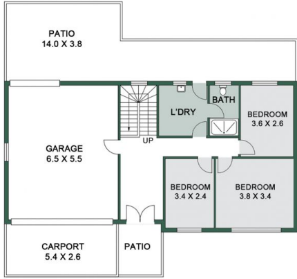
Lower Floor
